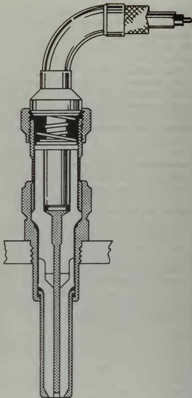
FIGURE 4-79. Constrained-gap igniter plug.
